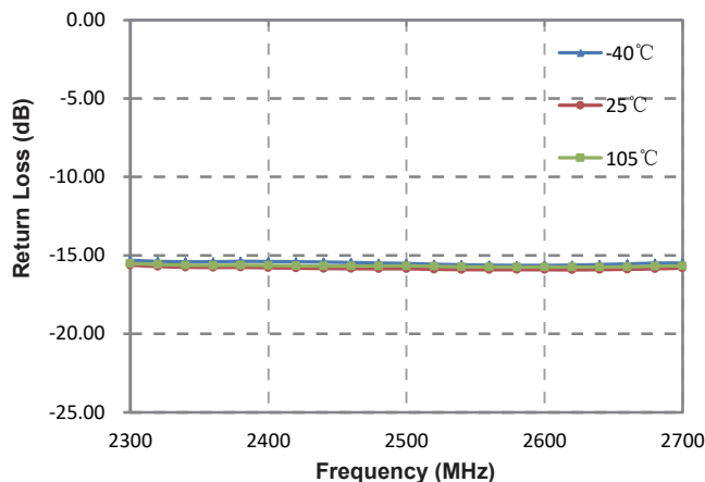
Return Loss (Port 3)
