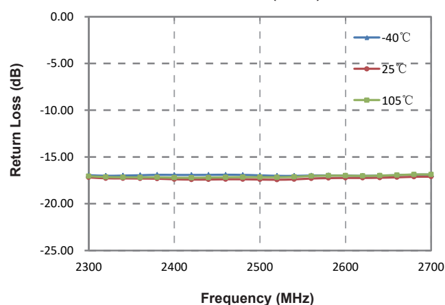
Return Loss (Port 2)
